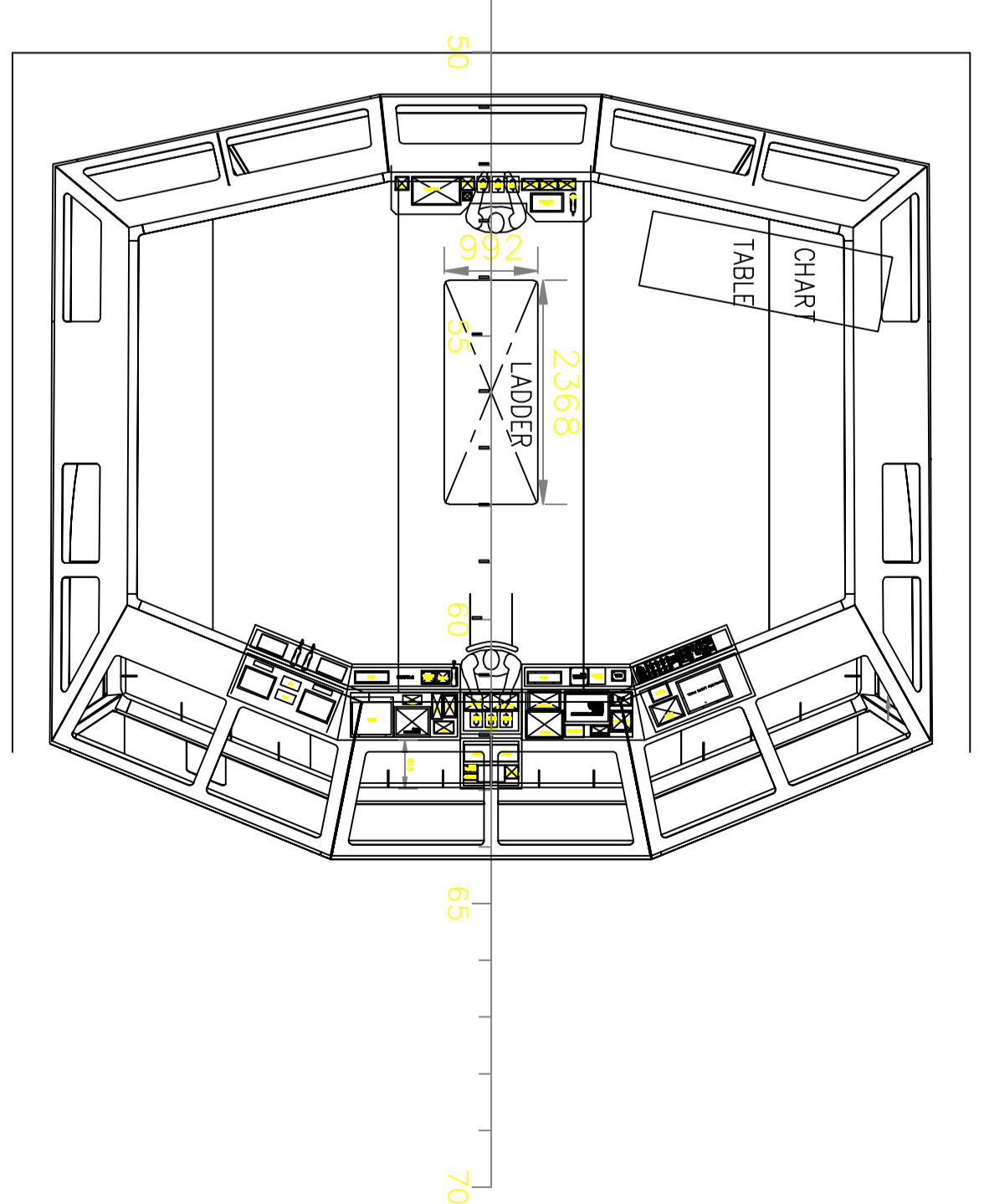
WHEELHOUSE DECK
