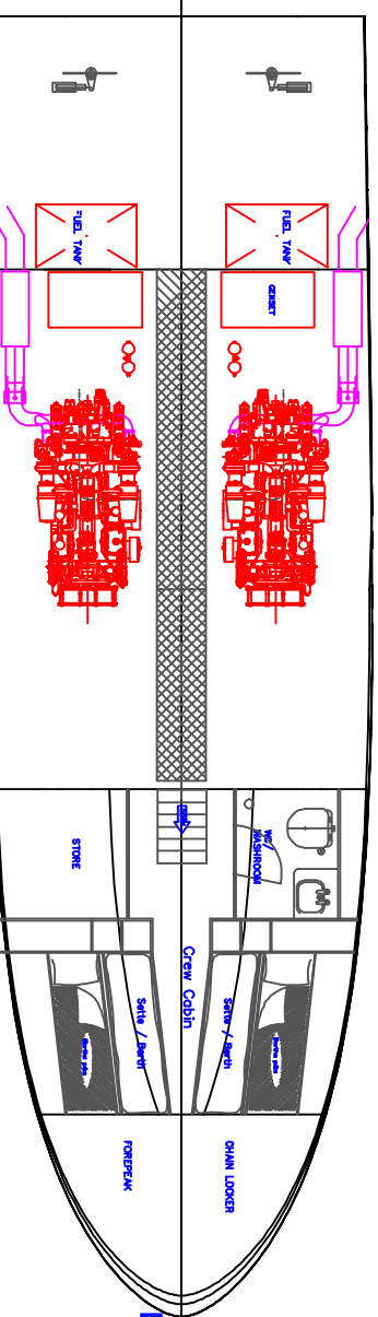
LOWER DECK PLAN
