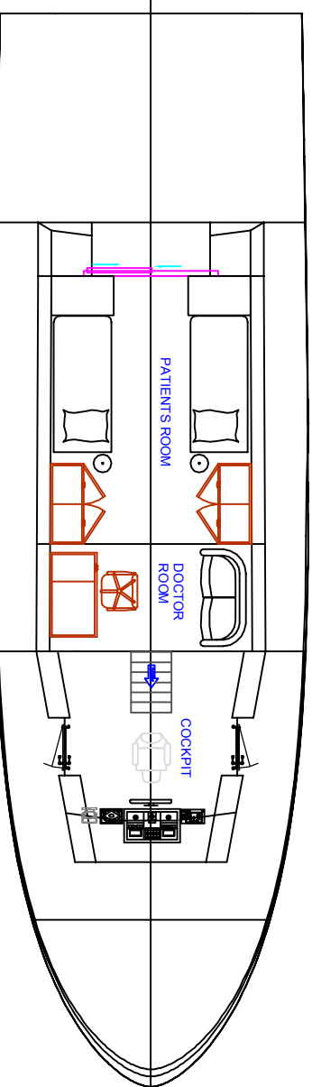
MAIN DECK PLAN
